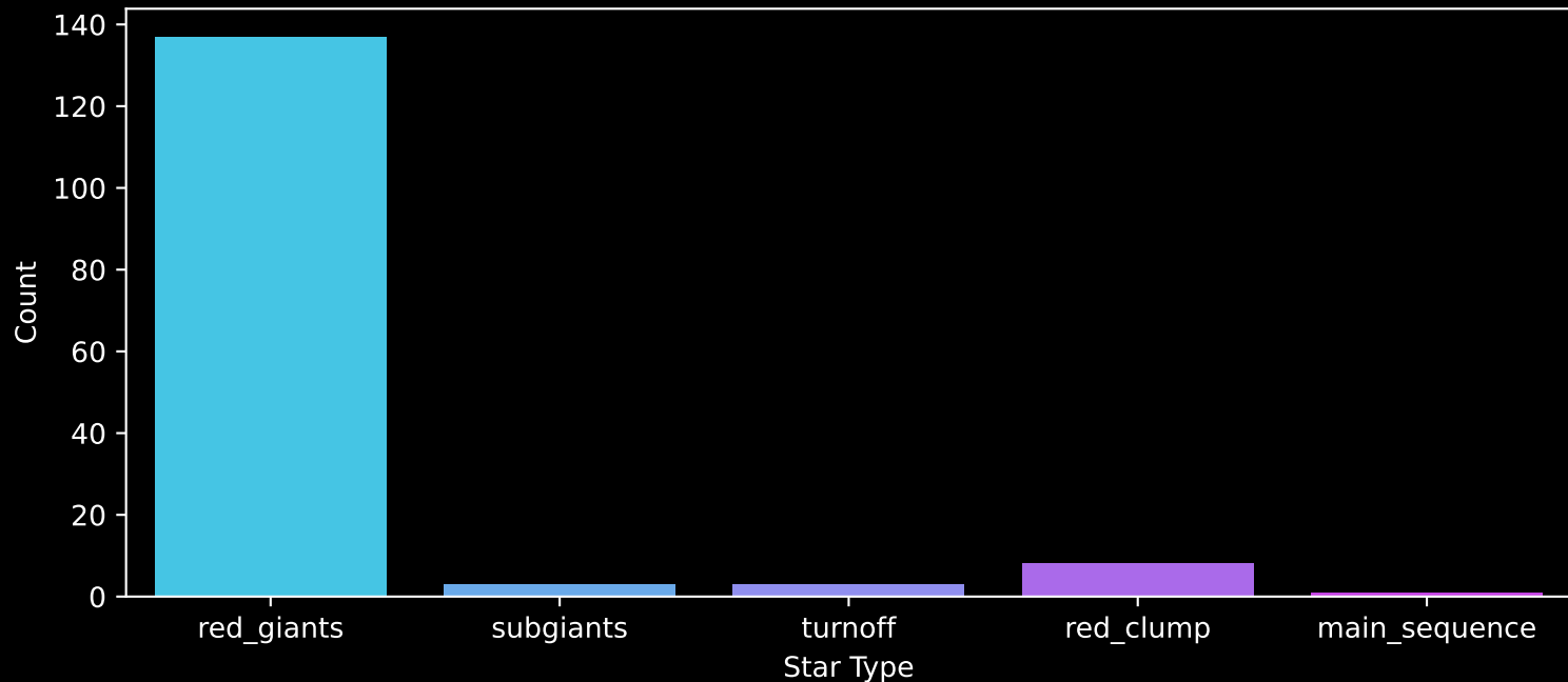
APOGEE DR17 Field: [Per_W] Count plot of Star Type
