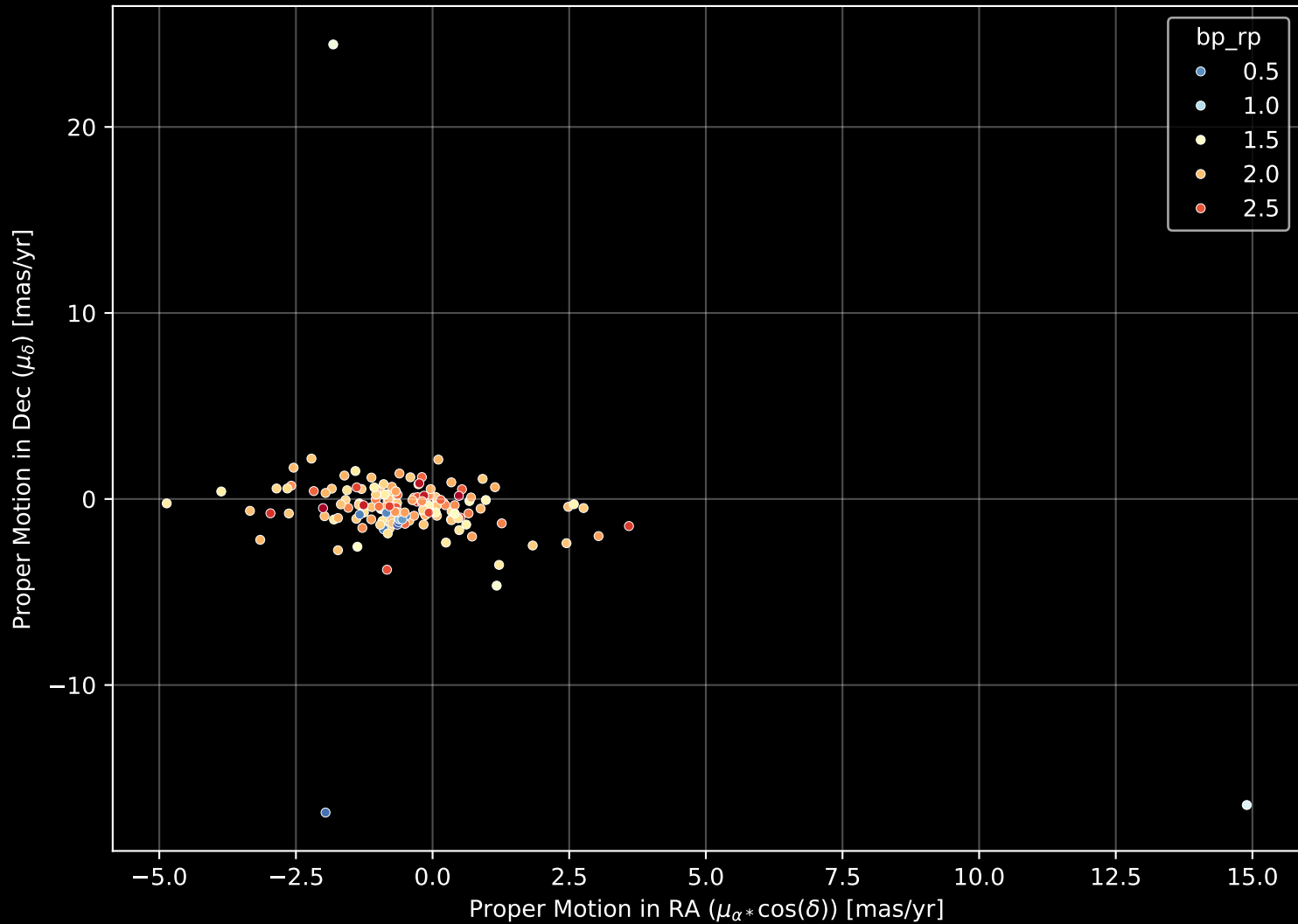
APOGEE DR17 Field: [Per_W] Proper Motion Diagram (n= 152)
