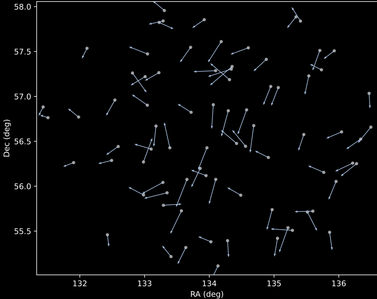
APOGEE DR17 Cluster 1 Proper Motion Vectors (n=78)
