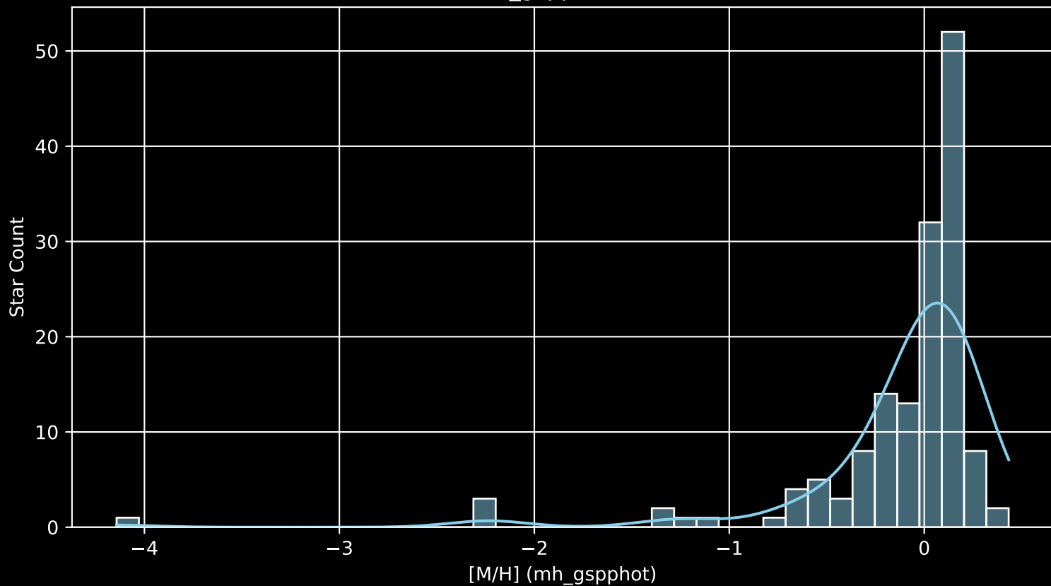
APOGEE DR17 Field: [Per_W [M/H] (mh_gspphot) (n= 150)
