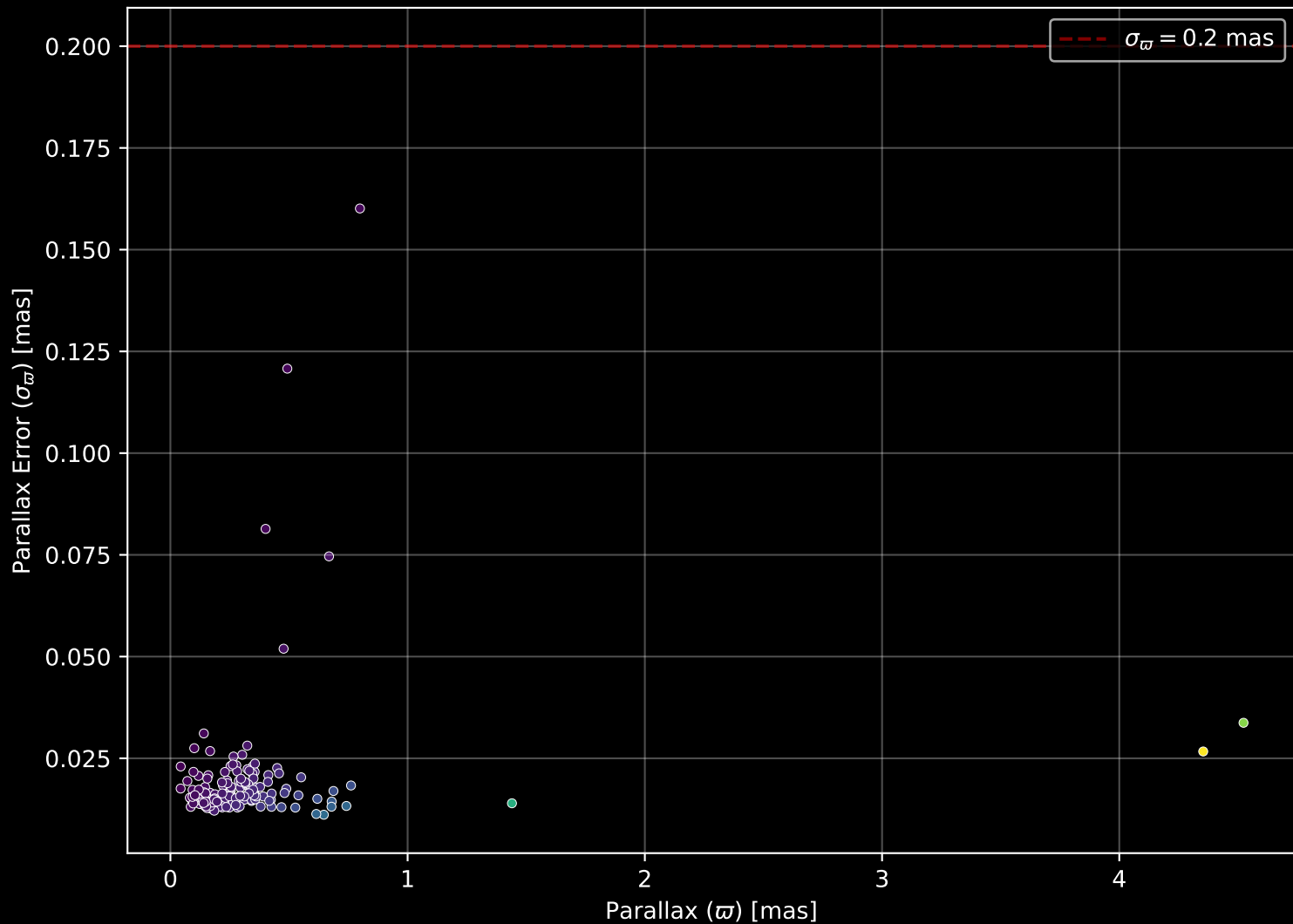
APOGEE DR17 Field: [Per_W] Parallax Quality (n= 152)
