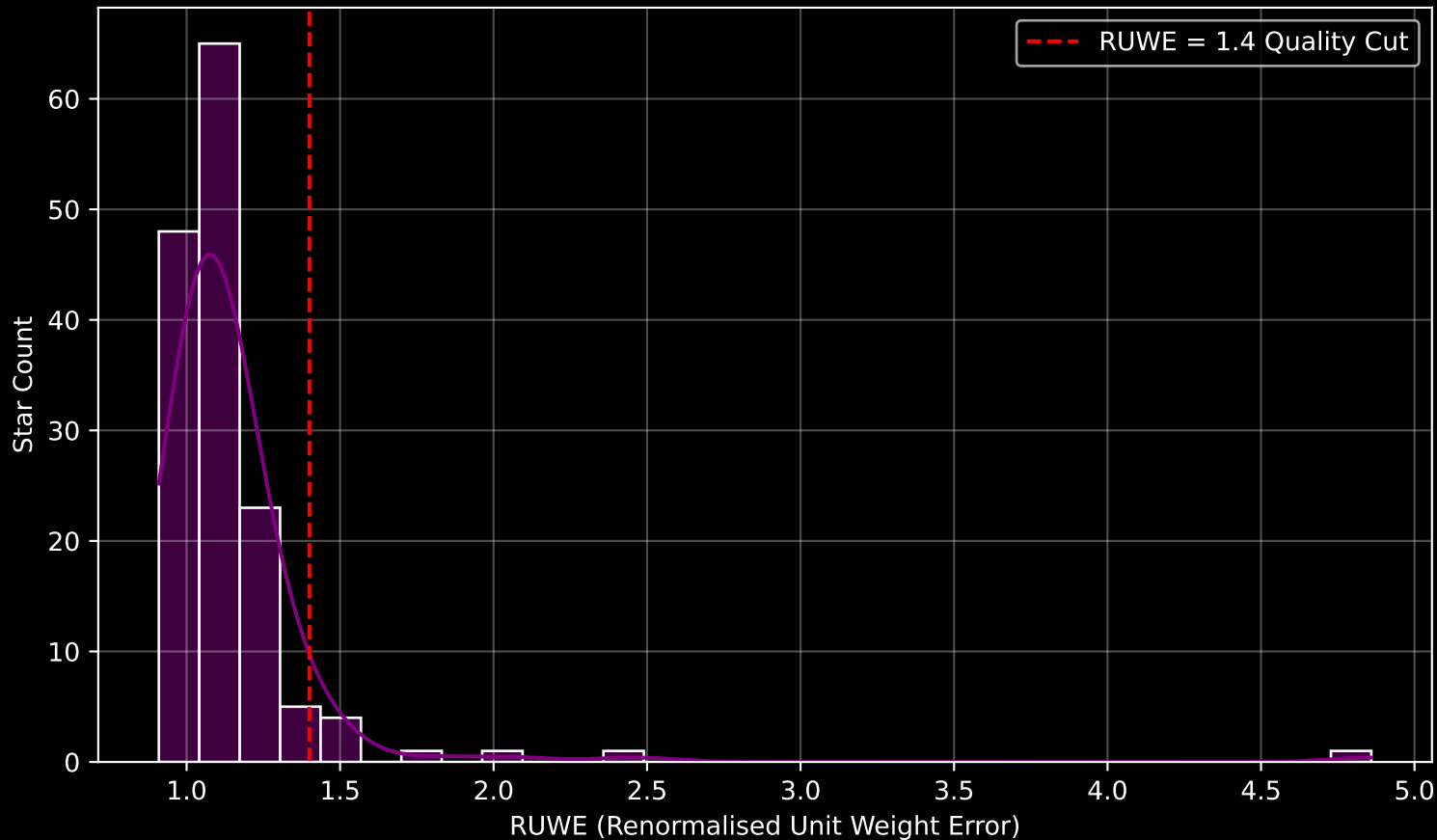
GAPOGEE DR17 Field [Per_W] RUWE Distribution (n= 149)
