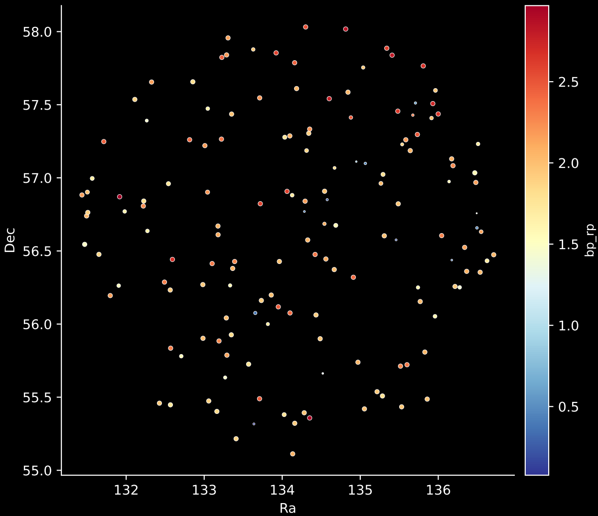
APOGEE DR17 Field: [Per_W] Stars: 152
